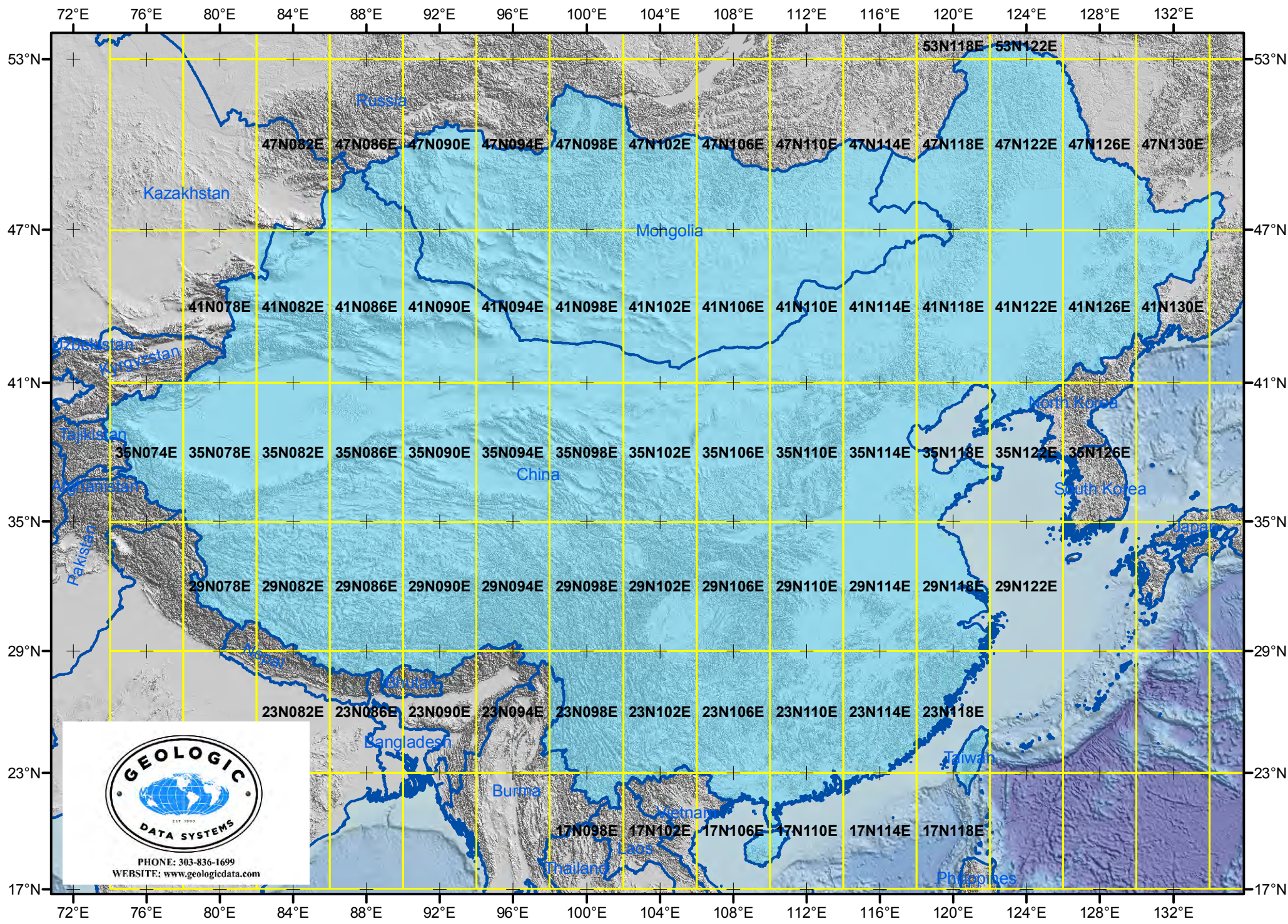
Index for the 1:500,000 scale China-Mongolia Geologic Mapping Project (blue wash) Yellow outline shows 500,000 scale sheets, numbered based on the lower left coordinate.
