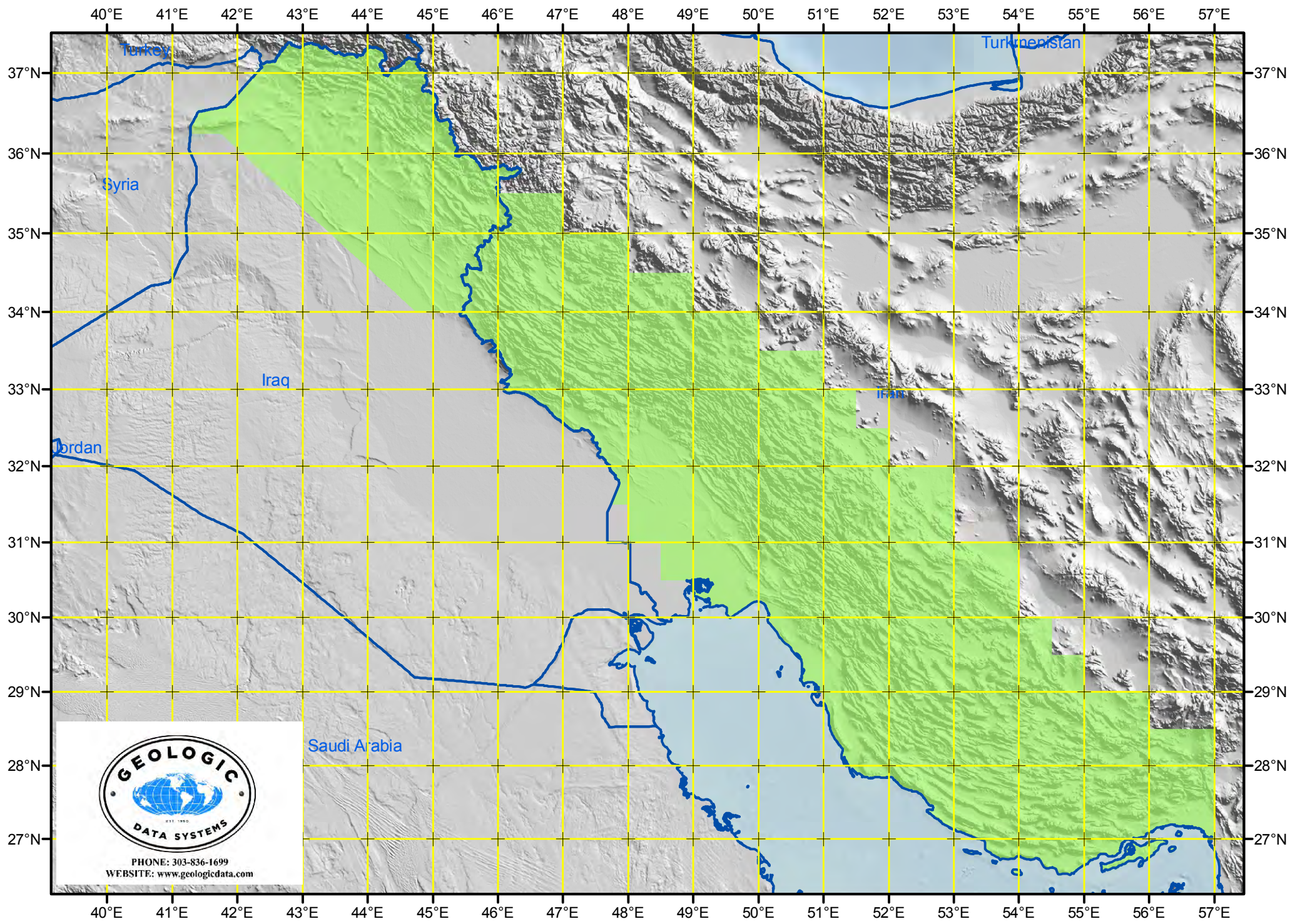
Index for the 1:100,000 scale Iran-Iraq Zagros Region Geologic Mapping Project. Yellow outline shows 100,000 scale 1°x1° sheets, numbered based on the lower left coordinate.
